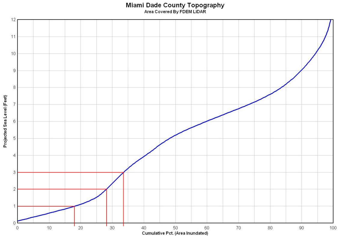
Figure 4. Hypsographic (hypsothetic) Curve Showing the Distribution of Land Elevation for Urban Miami-Dade County. This chart illustrates the percentage of the eastern two-thirds of Miami-Dade County’s land area that would be below sea level for any given sea level rise scenario based on LiDAR elevation data. The red lines connect the percentage of land for each foot of rise up to 3 feet (see Table 8). Just as sea level rise this century is expected to be non-linear, so will the percentage of land impacted at each sea level rise increment. Certain specific sea level rise horizons will require greater adaptation efforts than others. The Everglades portion of the County (about 1/3 of the total County area) was not covered by the LiDAR data source but adding it would make the left half of the curve lower and significantly increase the percentage of land impacted in the early part of sea level rise (Source: P. W. Harlem, Florida International University – by permission).
